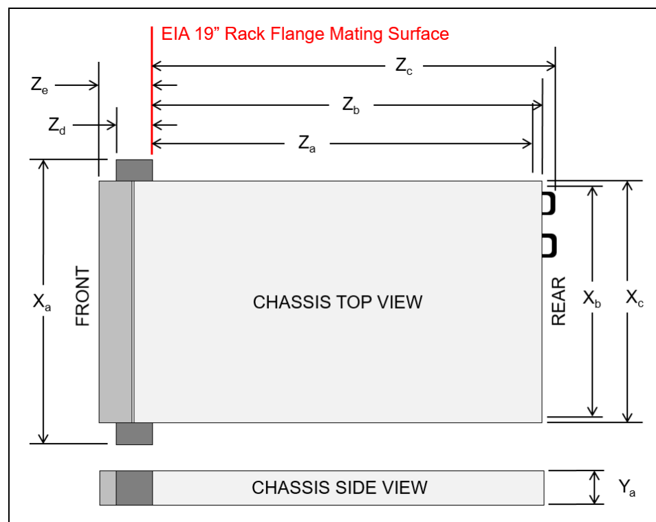
Figure 26. Server dimensions
