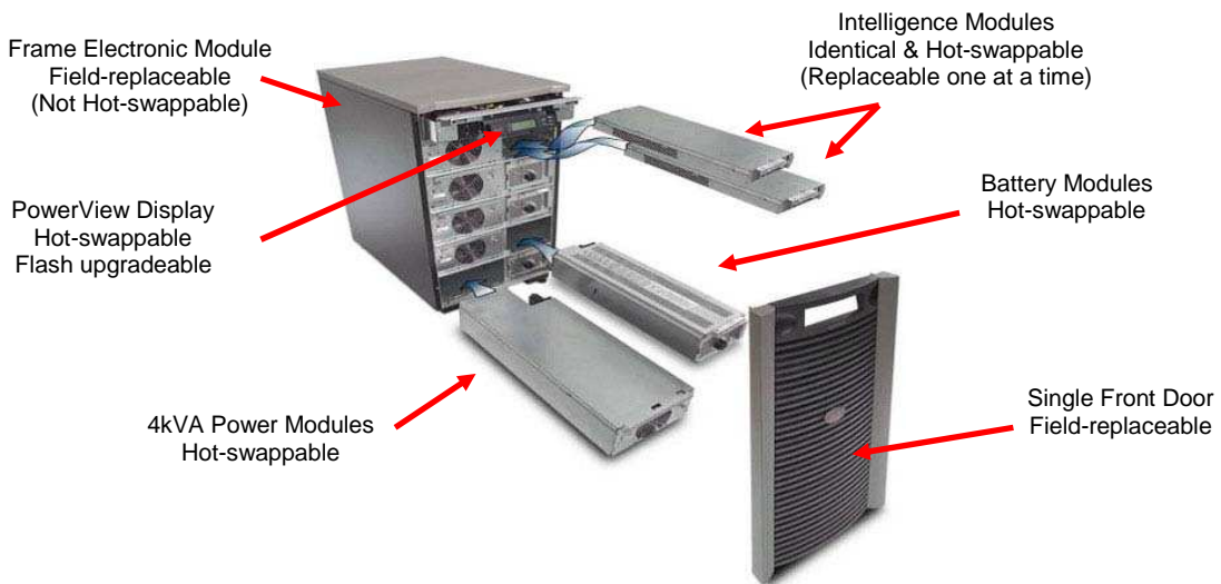
SYA16K16RMI, (Single phase 230V or three phase 400V)
