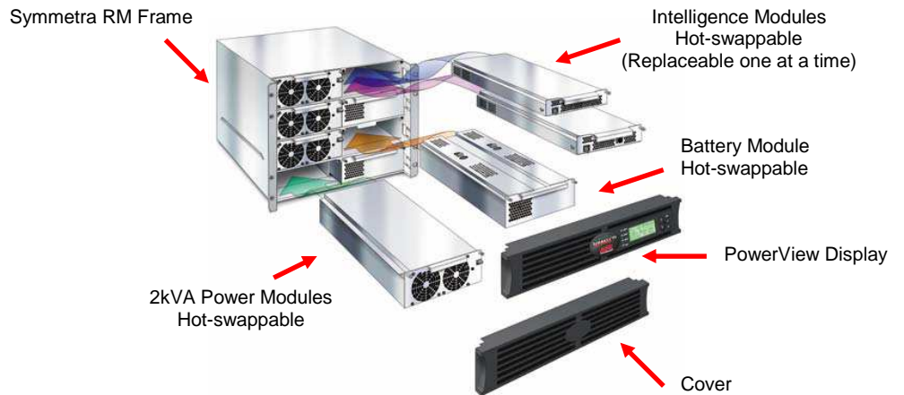
SYH6K6RMI, (Single phase 230V)
